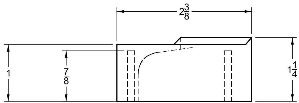
Right View
