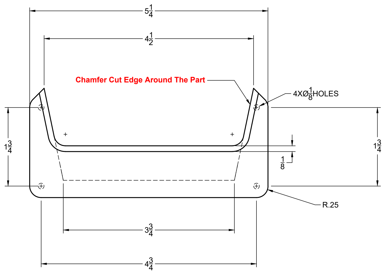
Top View
